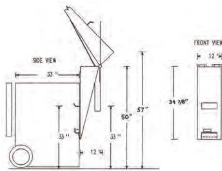
Part No: M-5000005-M Mounts 50" Loading Height
