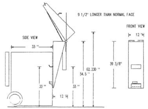
Part No: M-5000005-EX Mounts 54.5" Loading Height
