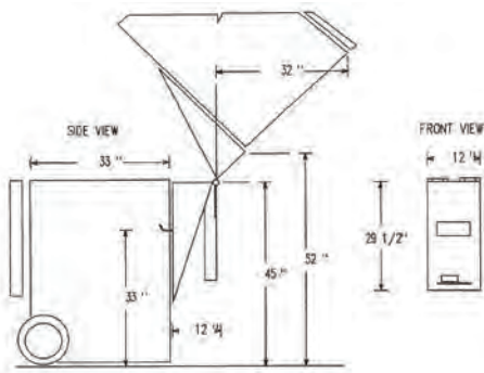
Part No: M-DBB-501C Mounts 45" Loading Height
